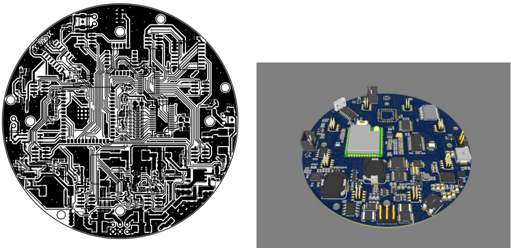
Main board PCB layout (top copper) and 3D populated render
